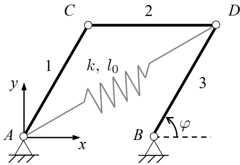
Figure 1: A four-bar linkage with a spring
